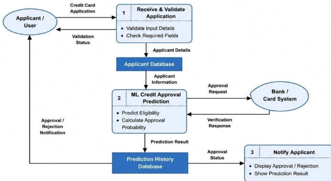
Figure 1: Level 1 DFD for Credit Card Approval Prediction
